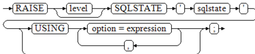
图 11-36 raise_sqlstate::=
