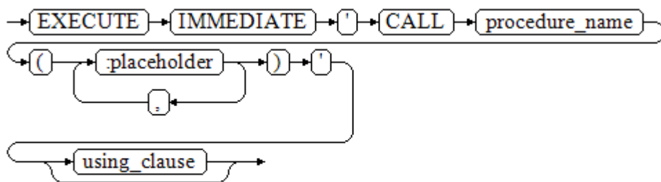
图 11-11 call_procedure::=
