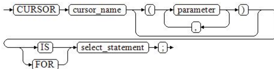
图 11-26 static_cursor_define::=
