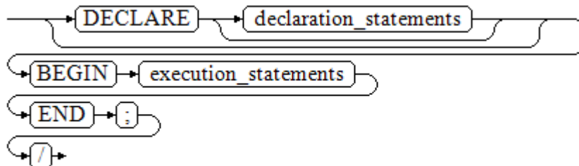
图 11-2 anonymous_block::=
